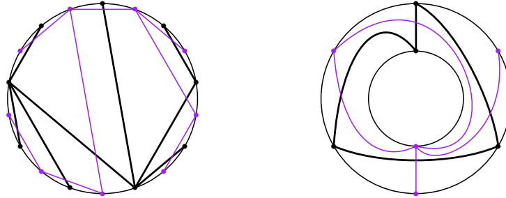
Figure 16. Properly embedded tree (left) and unicycle (right).
