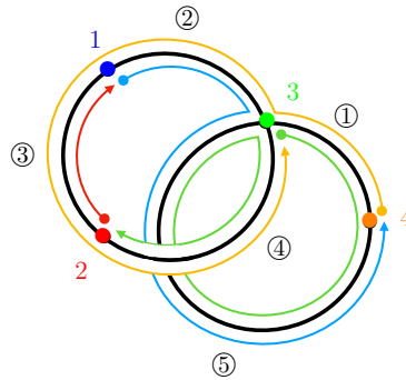
Figure 2. The graph from Figure 1 with its migts.
