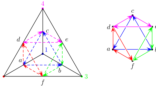
Figure 20. An embedded K_4 and its medial digraph.
