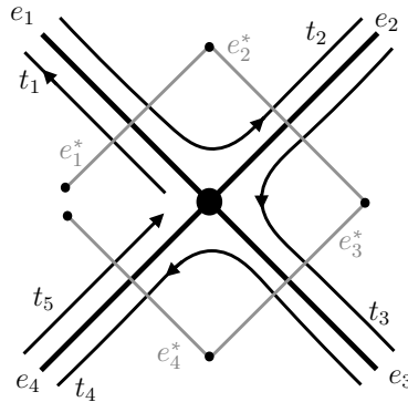
Figure 4. The local structure of migts.
