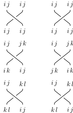
Figure 10. The Hurwitz action on factorizations.
