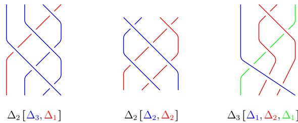
Figure 14. \Delta_4 .
