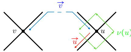
Figure 5. \mu(\Gamma^*) = \mu(\Gamma)^{-1} .
