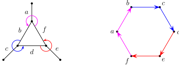
Figure 7. A non-e-realizable leo and its medial digraph.
