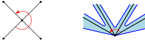
Figure 17. Thickening the star of a vertex.
