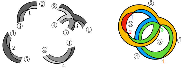
Figure 18. The peg of the e-v-graph of Figure 1.
