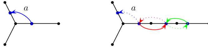
Figure 23. Subdividing to get a diverse FAS.
