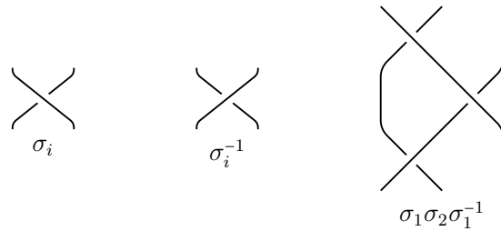
Figure 9. Generators and multiplication in the braid group.
