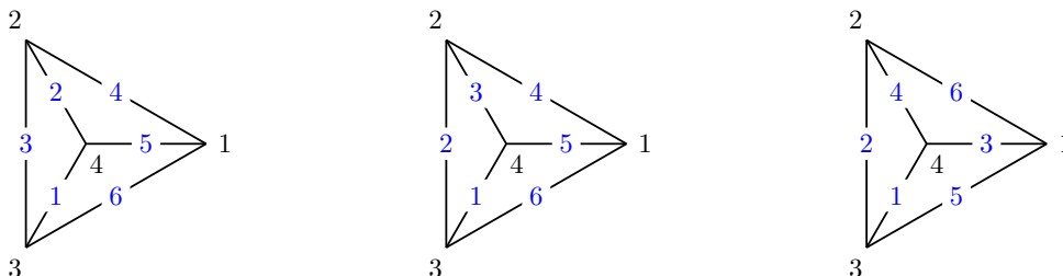
Figure 25. Proof of Theorem 4.22 for n = 4 : \mu = (1, 2, 3) (left), \mu = (1, 2)(3, 4) (center) and \mu = \text{id} (right).
