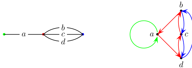
Figure 22. A nonpeggable ceg and its medial digraph.
